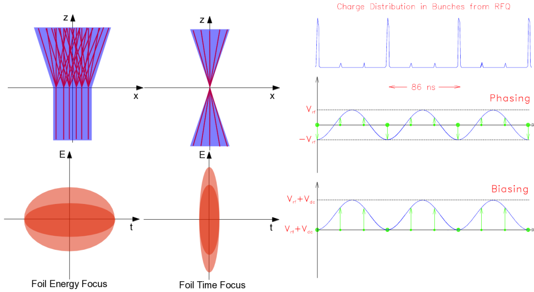
Figure 5: top left: Effects of stripping foil on beam geometry, for z being the beam axis and x being transverse (also valid for y ). Note the increase of emittance for the unfocussed case - each point on the foil surface can be considered a point source of beam, which complicates beam transport downstream. bottom left: Energy-time (longitudinal) phase space of beam before (dark red) after (light red) foil interaction. right: Schematic representation of the main buckets and both satellites. The 11MHz chopper RF is shown in the centre graph, and the chopper RF + chopper plate DC offset is shown at the bottom. Note that the deflection field is 0 when the main bunch crosses the buncher.
